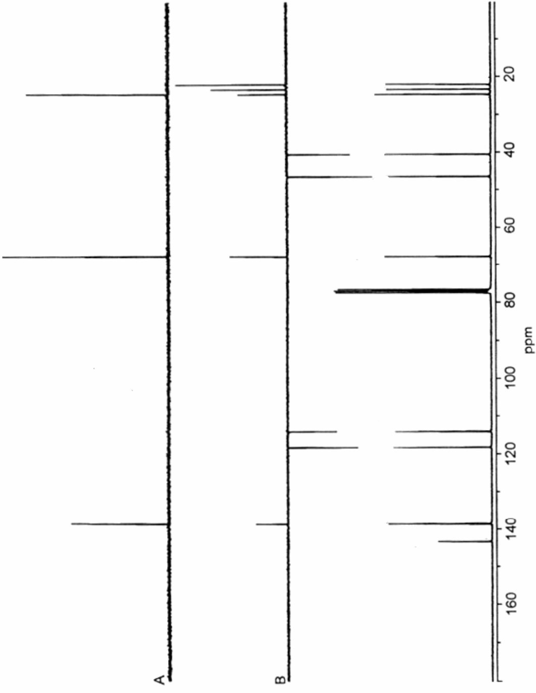
^{13}\text{C} data (A = DEPT-90, B = DEPT-135, bottom = standard ^{13}\text{C} )
